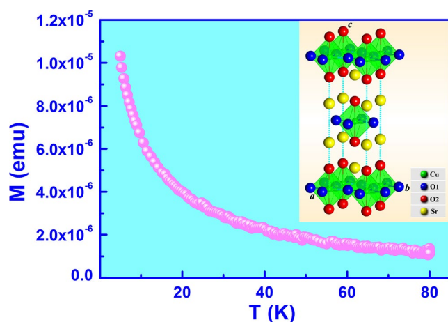
FIGURE 1 The temperature dependence of magnetization (M) curve after cooling in a 50 Oe magnetic field. The inset indicates the schematic view of the crystal structure of \text{Sr}_2\text{CuO}_{3+\delta} with the \text{K}_2\text{NiF}_4 type tetragonal structure containing [\text{CuO}_2] planes (O1) and the apical oxygen sites (O2) [Color figure can be viewed at wileyonlinelibrary.com ]
